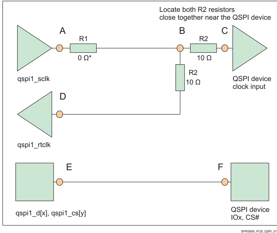
图 8-19. QSPI Interface High Level Schematic Mode 0 (POL=0, PHA=0)
