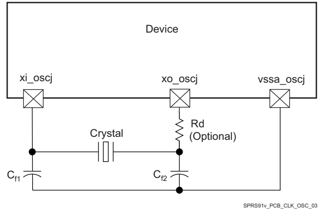
图 8-22. Grounding Scheme for High-Frequency Clock
