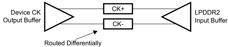
图 8-32. CK Signals Topology
