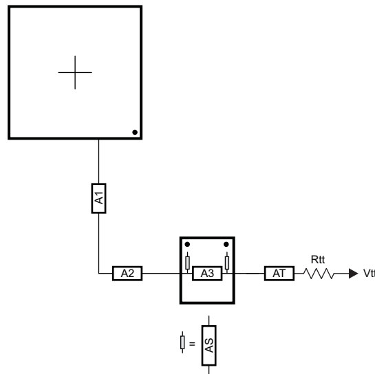
图 8-54. ADDR_CTRL Routing for Two Mirrored DDR3 Devices
