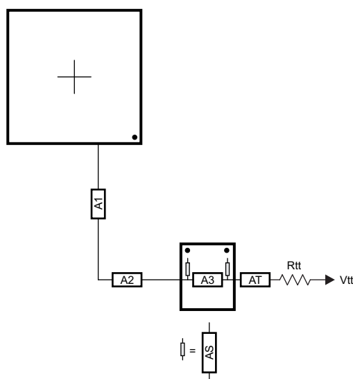
图 8-59. CK Routing for Two Mirrored DDR3 Devices
