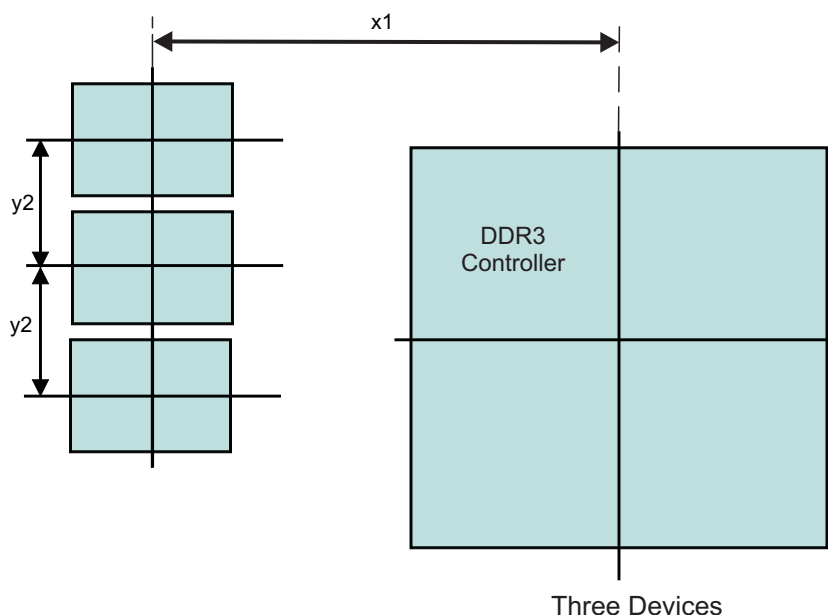
图 8-47. Placement Specifications
