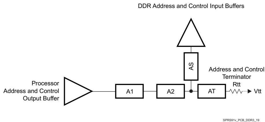
图 8-62. ADDR_CTRL Topology for One DDR3 Device
