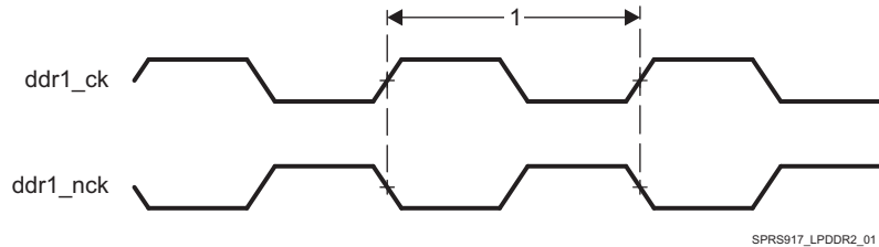
图 8-23. LPDDR2 Memory Interface Clock Timing
