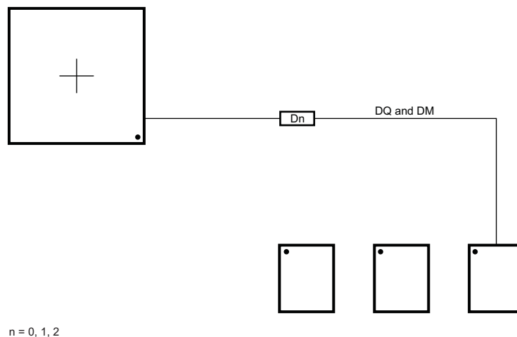
图 8-68. DQ/DM Routing With Any Number of Allowed DDR3 Devices
