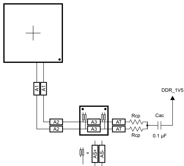
图 8-59. CK Routing for Two Mirrored DDR3 Devices
