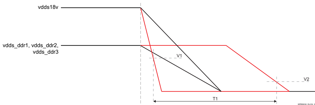
图 5-4. vdds18v and vdds_dds* Discharge Relationship (1)
