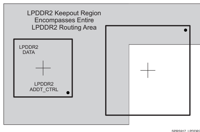
图 8-26. LPDDR2 Keepout Region
