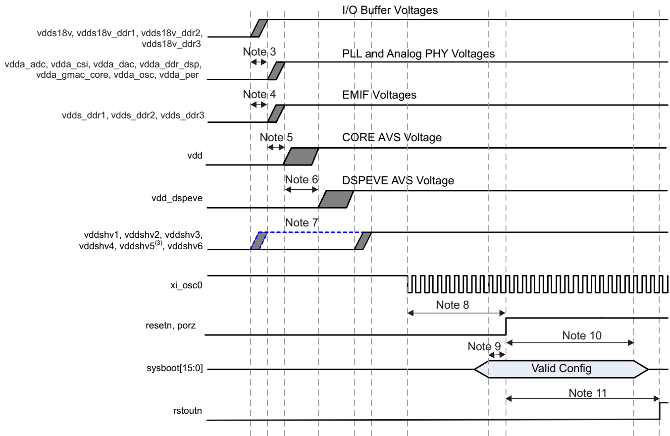
图 5-1. Power-Up Sequencing
