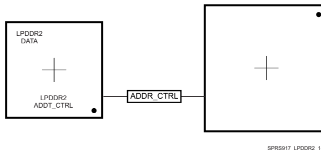
图 8-35. ADDR_CTRL Signals Routing
