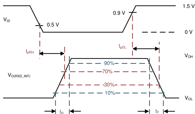
图 7-5. Receiver Test Circuit and Measurement
