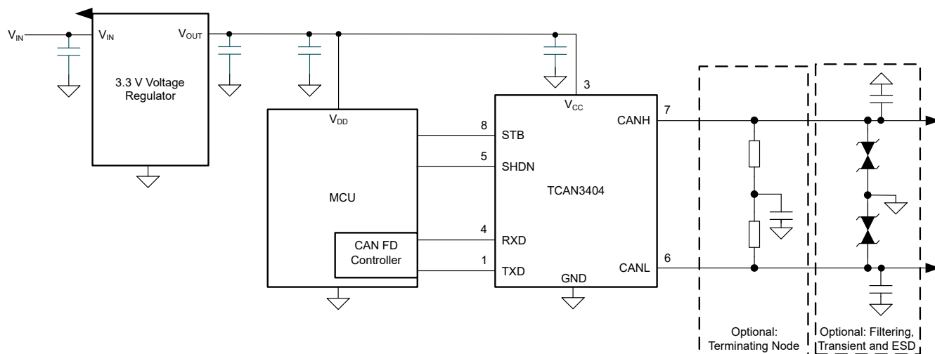
图 9-1. Transceiver Application Using 3.3V I/O Connections
