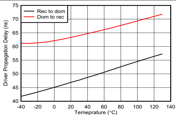
图 6-7. Driver Propagation Delay vs Temperature
