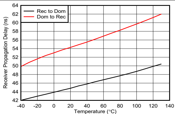
图 6-8. Receiver Propagation Delay vs Temperature
