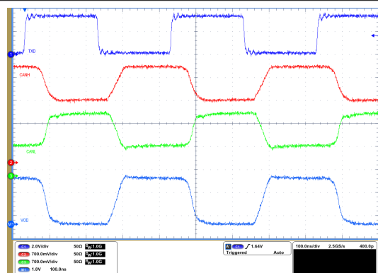
图 9-5. TXD_CANH_CANL_Vod waveforms for 60 \Omega load at 5Mbps toggling
