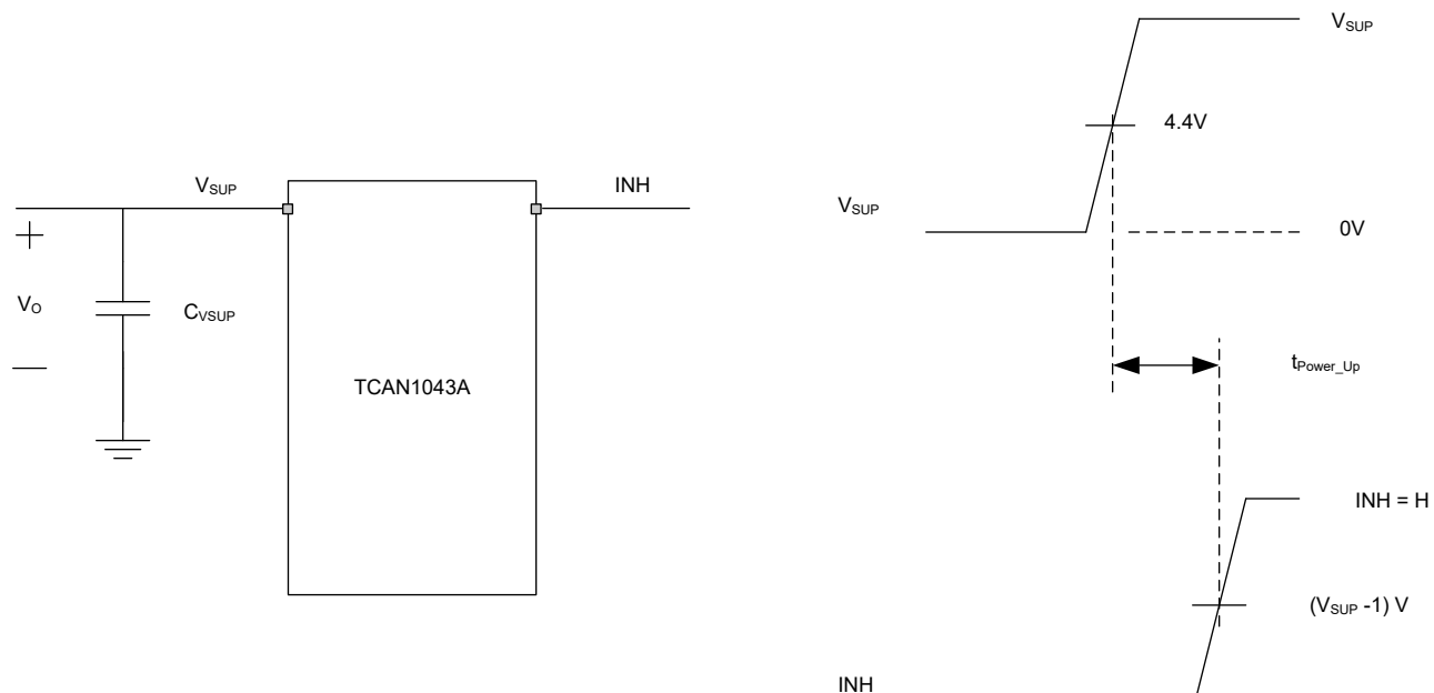
图 7-10. Power-Up Timing
