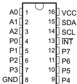
Pin Functions
