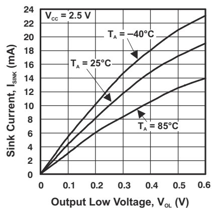
图 6-5. I/O Sink Current vs Output Low Voltage
