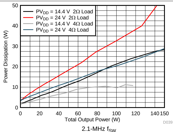
图 34. Power Dissipation vs Output Power
