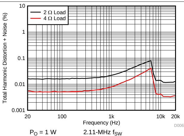
图 5. THD+N vs Frequency
