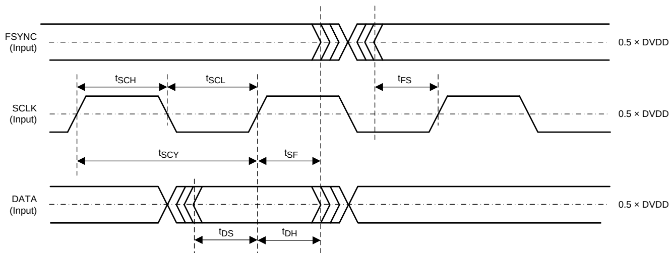
图 36. Serial Audio Timing
