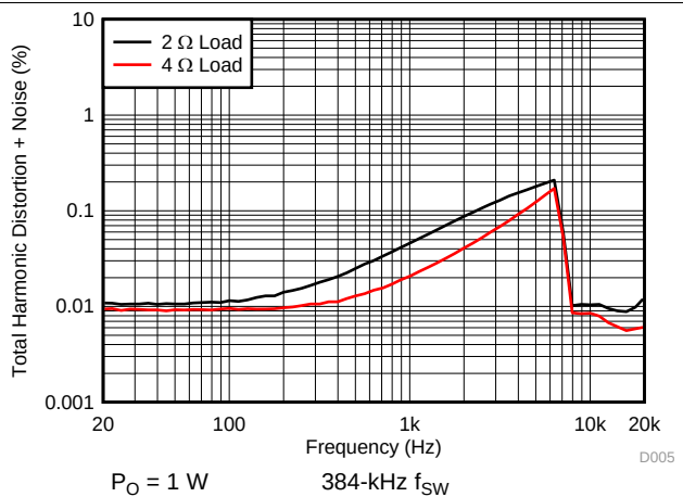
图 4. THD+N vs Frequency
