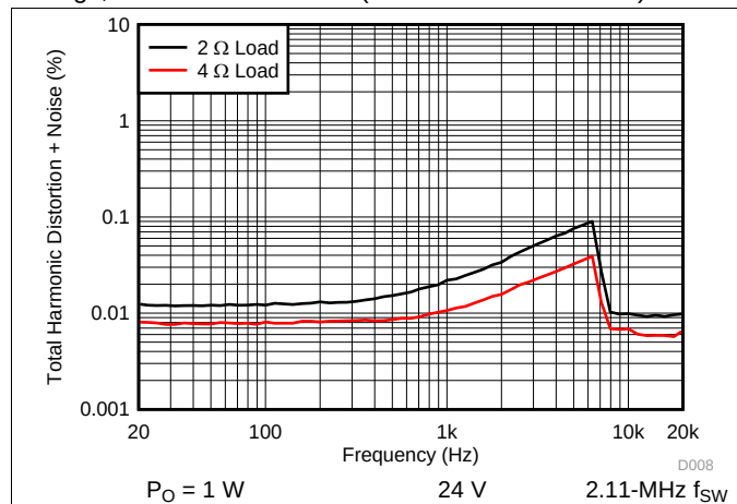
图 7. THD+N vs Frequency
