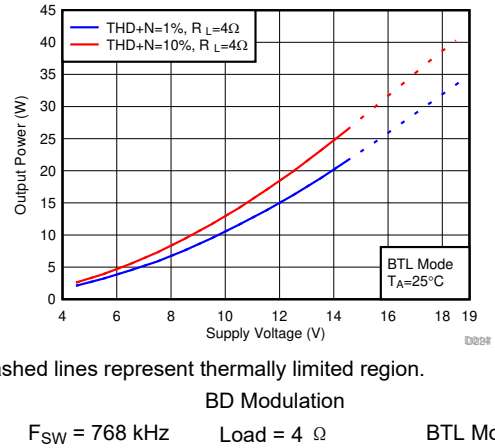
图 7-55. Output Power vs Supply Voltage
