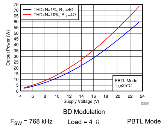
图 7-74. Output Power vs Supply Voltage
