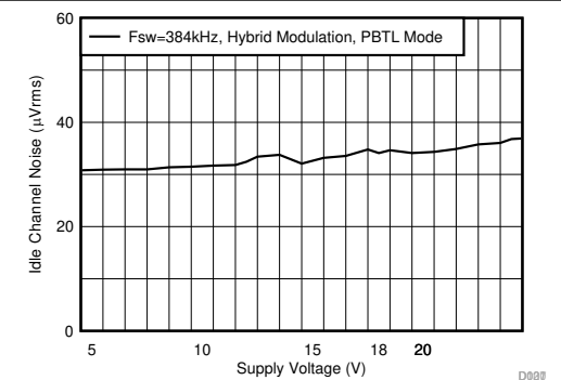
Hybrid Modulation F SW = 384 kHz Load = 6 Ω PBTL Mode
