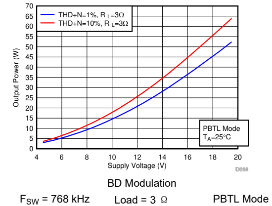
图 7-73. Output Power vs Supply Voltage
