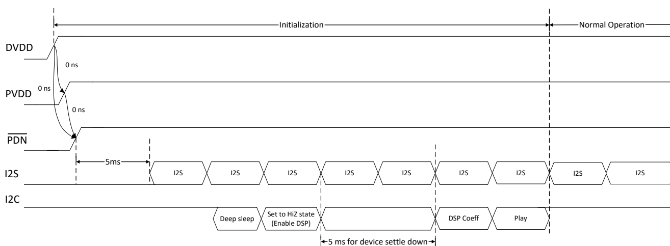
图 80. Start-up Sequence
