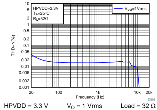
图 56. THD+N vs Frequency
