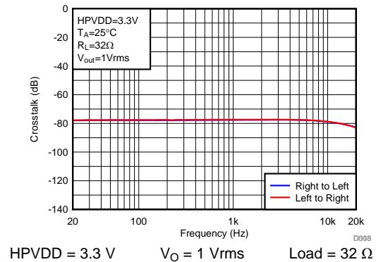
图 58. Crosstalk vs Frequency
