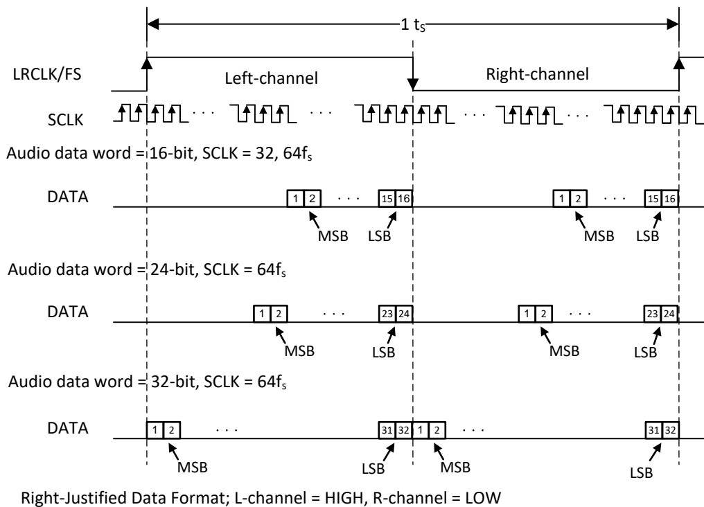
图 69. Right Justified Audio Data Format
