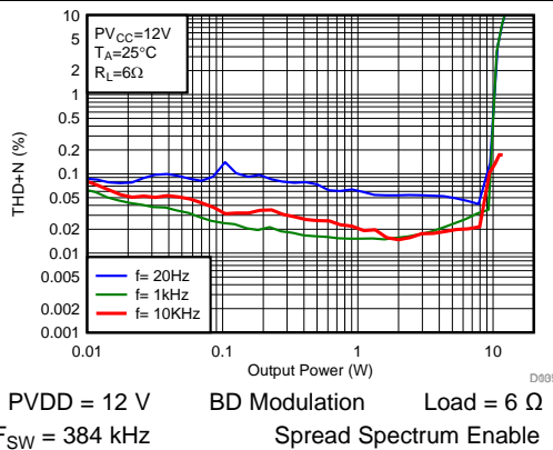
图 36. THD+N vs Output Power
