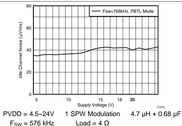
图 51. Idle Channel Noise vs Supply Voltage
