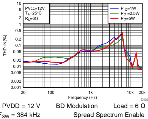
图 32. THD+N vs Frequency
