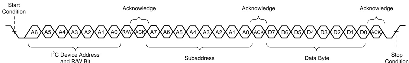
图 64. Random Write Transfer
