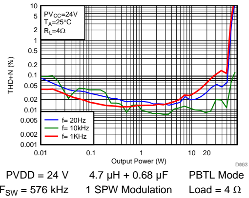
图 122. THD+N vs Output Power
