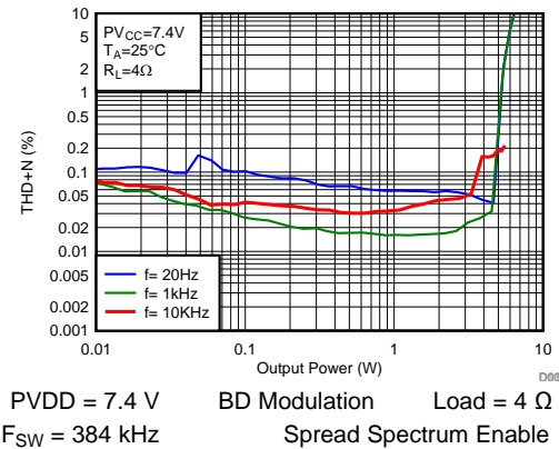
图 35. THD+N vs Output Power
