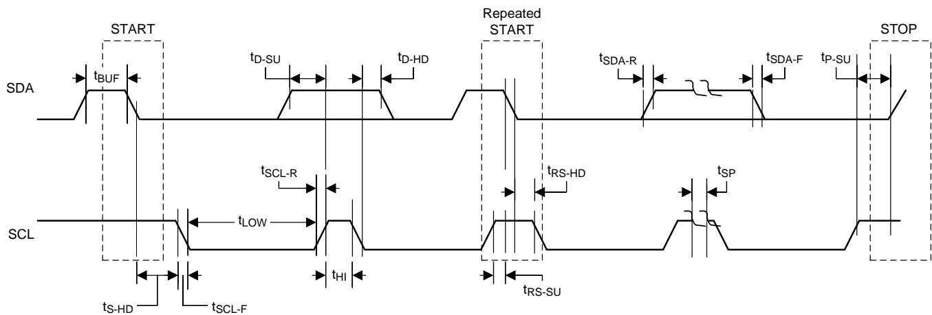
图 54. I²C Communication Port Timing Diagram
