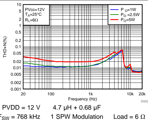
图 116. THD+N vs Frequency
