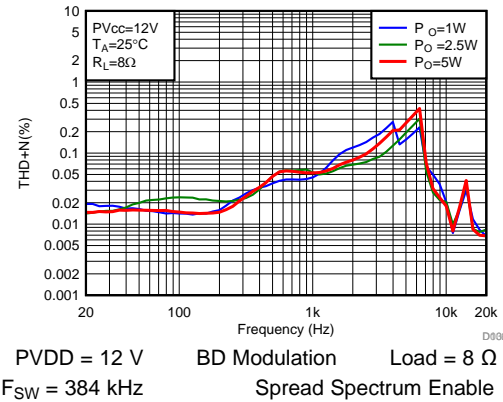
图 33. THD+N vs Frequency
