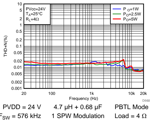
图 121. THD+N vs Frequency
