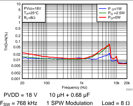
图 117. THD+N vs Frequency
