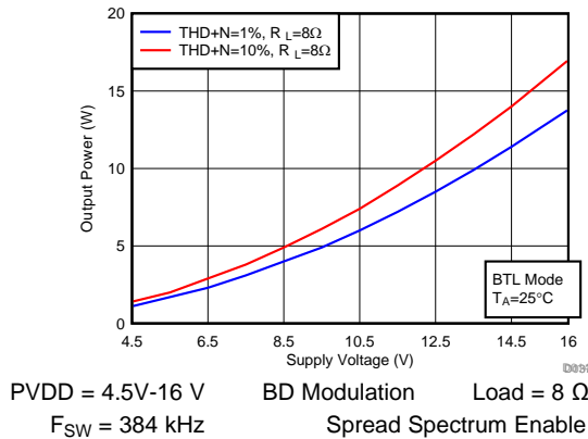
图 34. Output Power vs Supply Voltage
