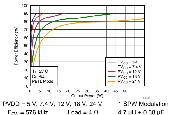
图 52. Efficiency vs Output Power
