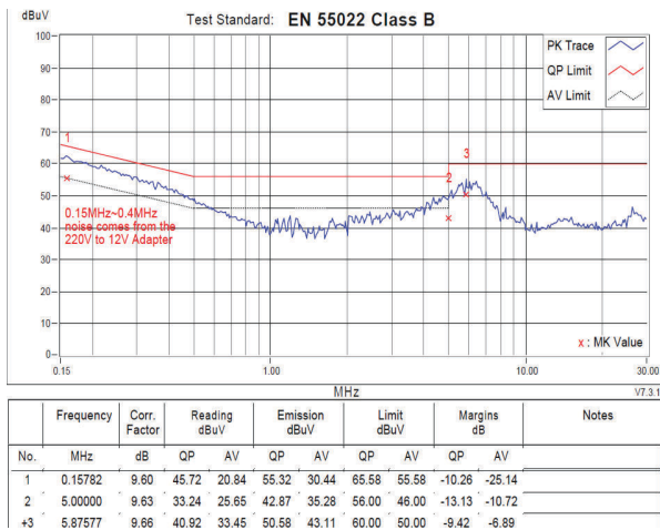
图 8-5. Conducted Emission with Ferrite Bead Filter - Line
