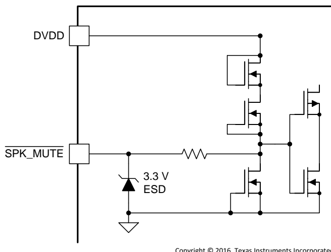
Figure 12. \overline{\text{SPK\_MUTE}} Pin
