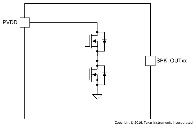
Figure 4. SPK_OUTxx Pins
