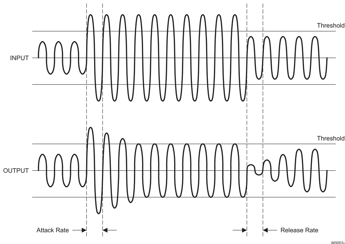
Figure 83. AGL Attack and Release
