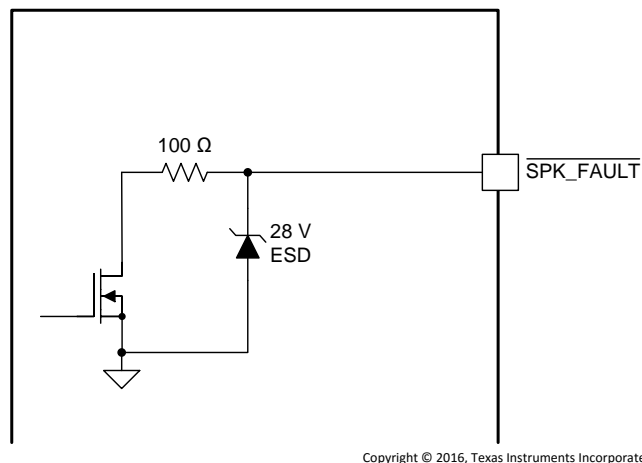
Figure 16. \overline{\text{SPK\_FAULT}} Pin
