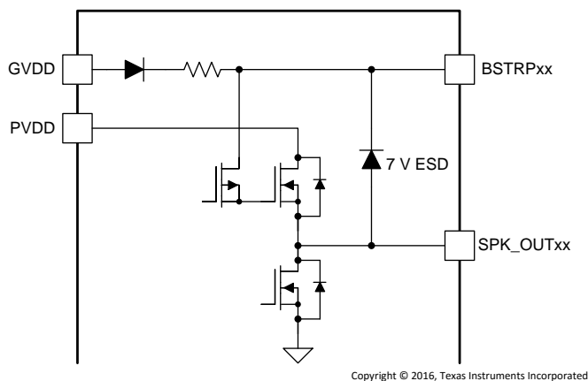
Figure 3. BSTRPxx Pins
