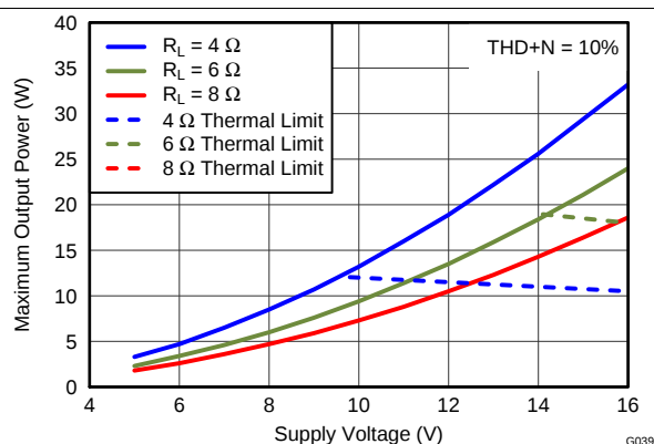
Figure 14. Output Power vs PVDD
