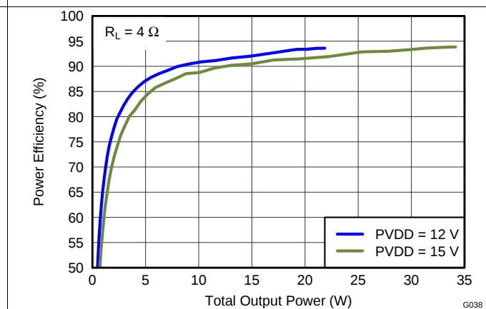
Figure 31. Efficiency vs Output Power
