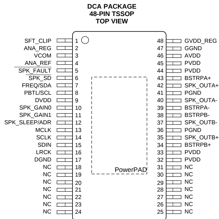
Pin Functions
