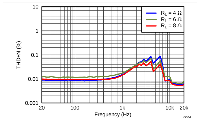
Figure 32. THD+N vs Frequency
