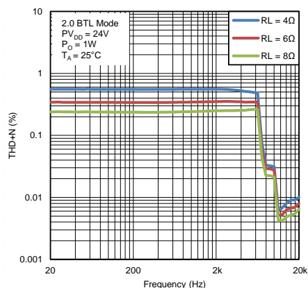
图 24. Total Harmonic Distortion vs Frequency
