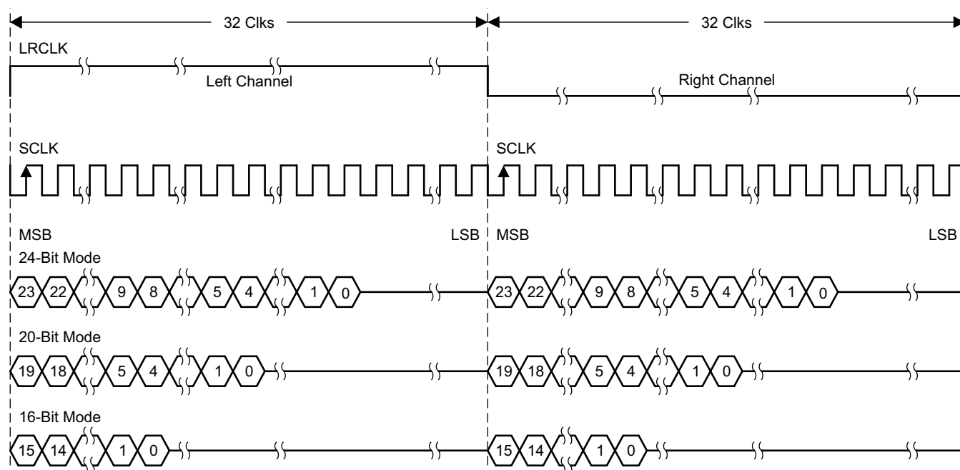
图 49. Left-Justified 64- F_s Format
