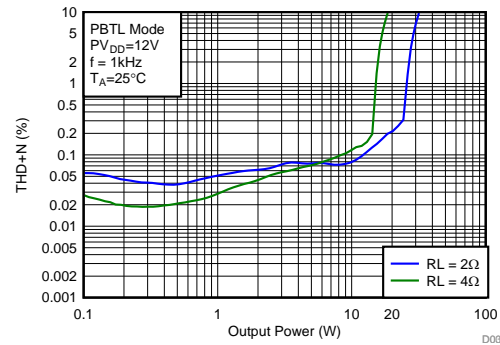
图 33. Total Harmonic Distortion + Noise vs Output Power (PBTL Mode)
