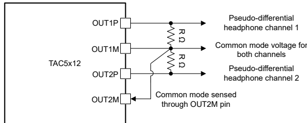
图 6-16. 带外部共模检测的伪差分输出连接 (OUT1x_CFG[2:0] = 3'b101)
