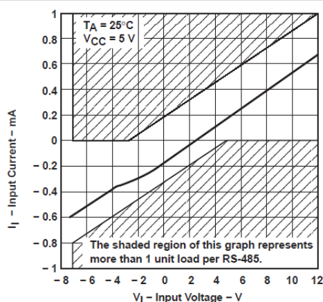
图 5-10. Receiver Input Current vs Input Voltage (Complementary Input at 0 V)
