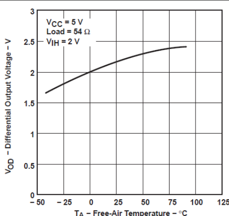
图 5-4. Driver Differential Output Voltage vs Free-Air Temperature
