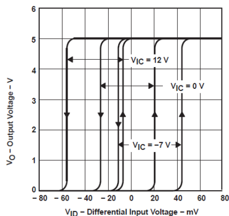
图 5-8. Receiver Output Voltage vs Differential Input Voltage
