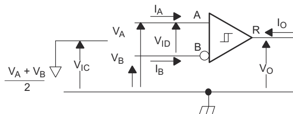
图 8-8. Receiver Voltage and Current Definitions
