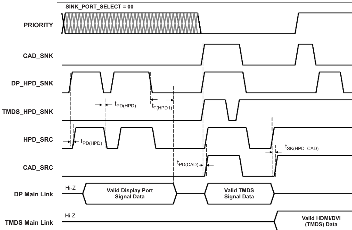
Figure 10. HPD and CAD Logic Description and Timing Diagram
