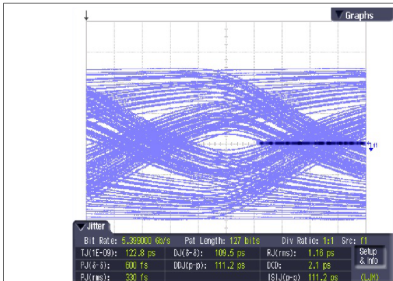
Figure 32. Main Link Input with 22-inch Trace; DisplayPort Sink
