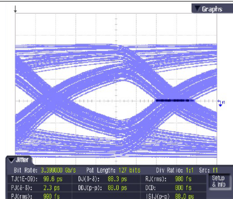
Figure 18. Main Link Input with 22-inch Trace; DisplayPort Sink
