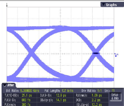
Figure 19. SN75DP126 Output; 22-inch Input Trace; 15 dB EQ Setting; DP Sink
