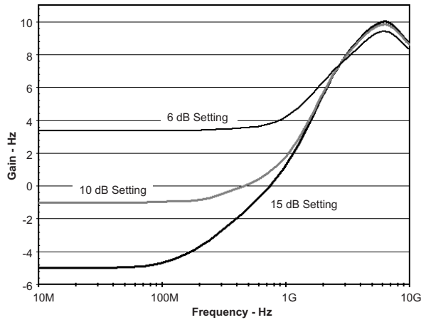
Figure 15. Typical EQ Gain Curves
