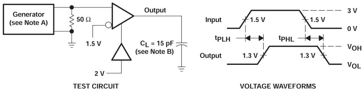
TEST CIRCUIT
