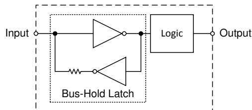
图 7-2. Bus-Hold circuit block diagram representation
