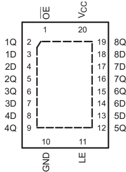
SN74LVC373A . . . RGY PACKAGE (TOP VIEW)
