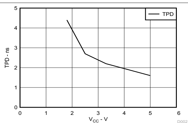
图 6-2. TPD Across V_{CC} at 25^\circ\text{C}
