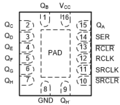
图 5-2. BQB Package 16-Pin WQFN Top View
