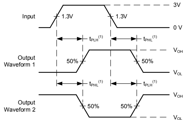
图 6-2. Voltage Waveforms, Propagation Delays for TTL-Compatible Inputs
