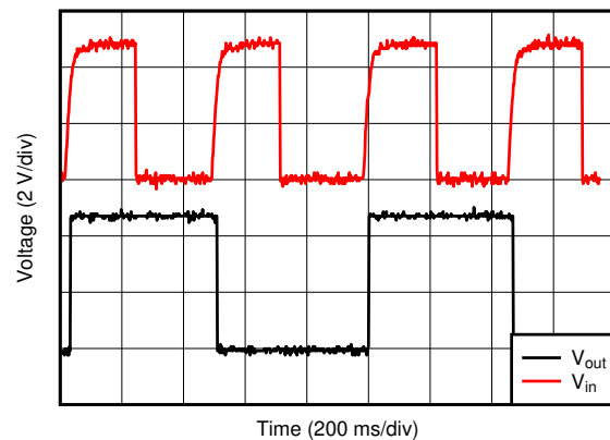
图 9-3. Circuit response with RC debounce V_{in} := \text{CLK input} , V_{out} := \text{Q output}
