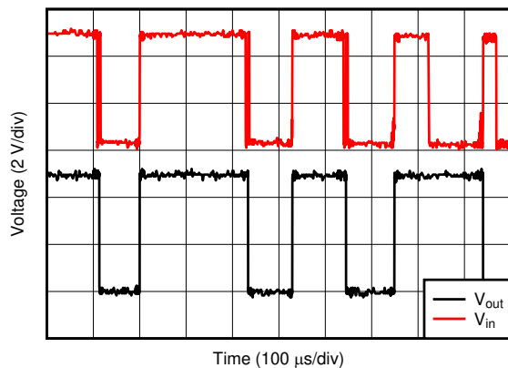
图 9-2. Circuit response without RC debounce V_{in} := \text{CLK input} , V_{out} := \text{Q output}
