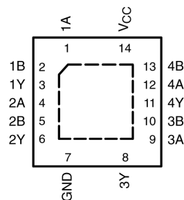
图 5-2. SN74AHCT00 RGY, BQA Package, 14-Pin QFN, WQFN (Transparent Top View)
