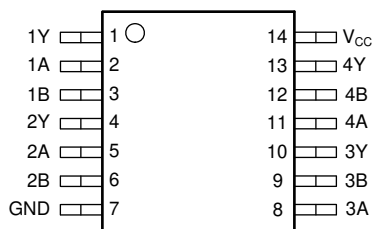
图 3-1. SN54AHC02 J or W Package, 14-Pin (Top View)
