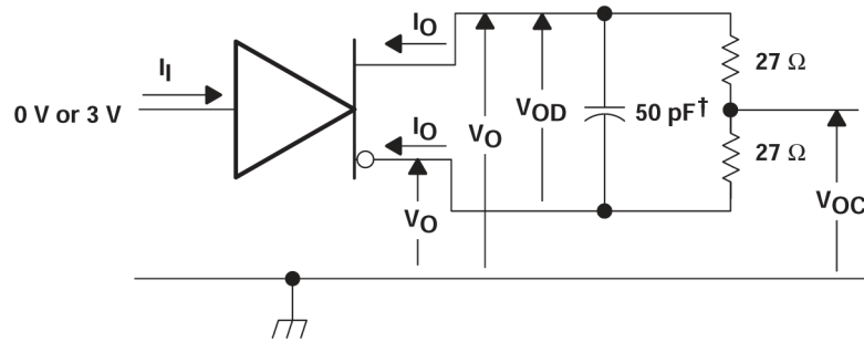
图 6-1. Driver Test Circuit, v_{OD} And v_{OC} Without Common-Mode Loading
