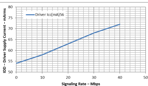
图 6-2. Driver Supply Current vs Signaling Rate
