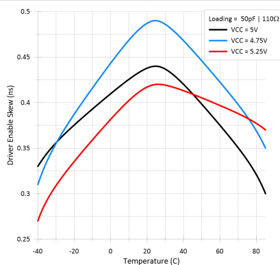
图 6-5. Driver Enable Skew vs Free-Air Temperature
