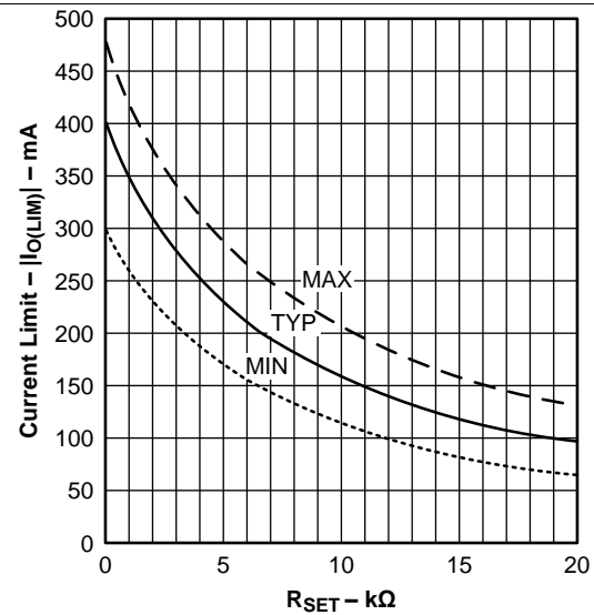
Figure 2. Typical Current Limit Characteristics
