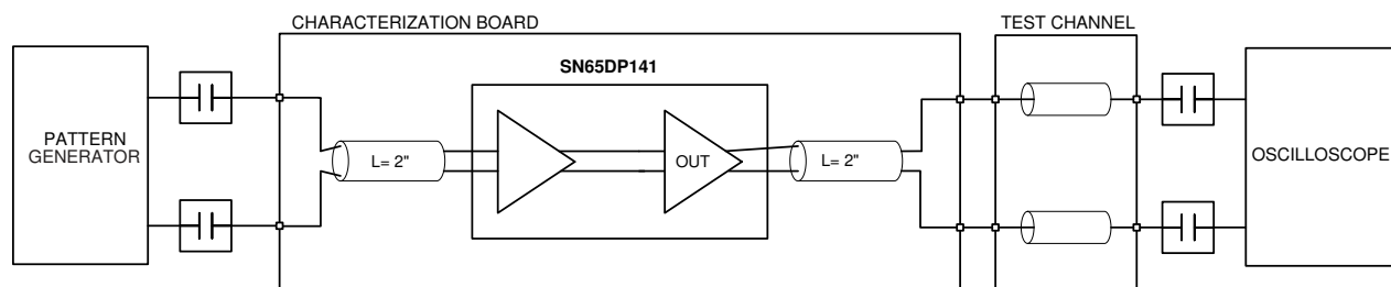
图 7-7. Transmit Side Performance Test Circuit
