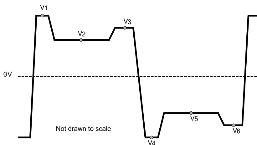
图 7-5. V_{(pre)} and V_{(post)} (test pattern is 1111111100000000 (8-1s, 8-0s))
