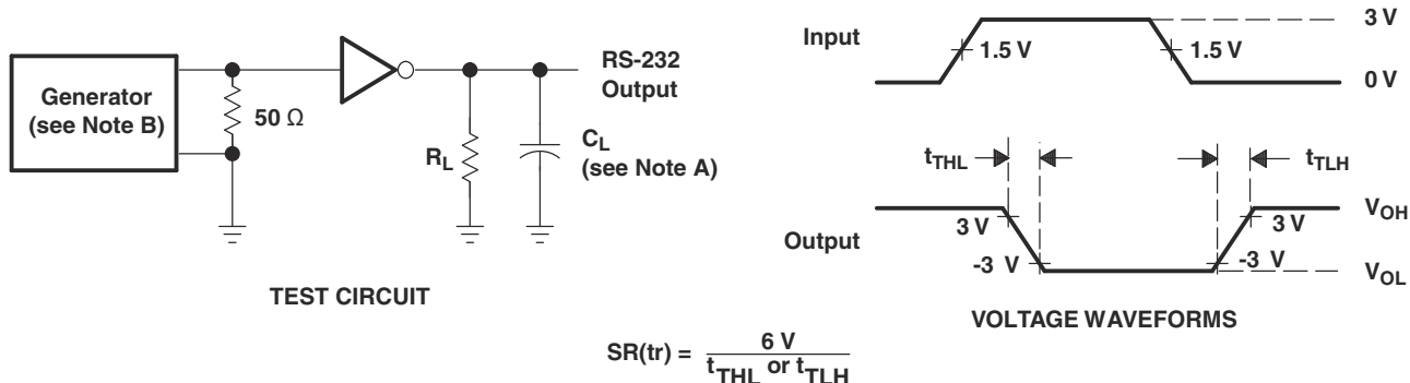
图 7-1. Driver Slew Rate
