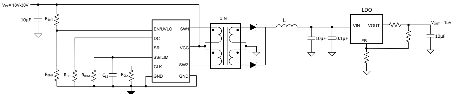
图 9-4. Typical Application Schematic for Wide-Ranging Input with Duty Cycle Control
