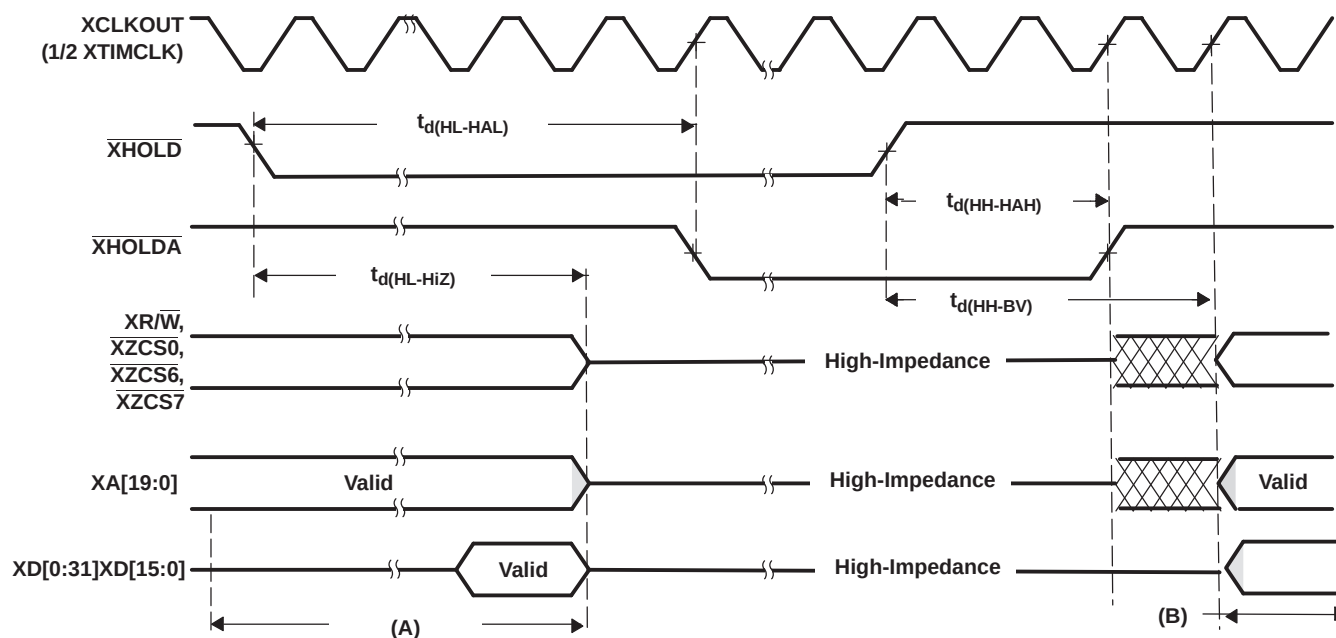
Figure 6-31. XHOLD/XHOLDA Timing Requirements (XCLKOUT = 1/2 XTIMCLK)
