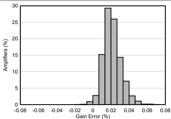
N = 1767 平均值 = 0.0124\% 标准偏差 = 0.0098\% G = 16\text{V/V}
