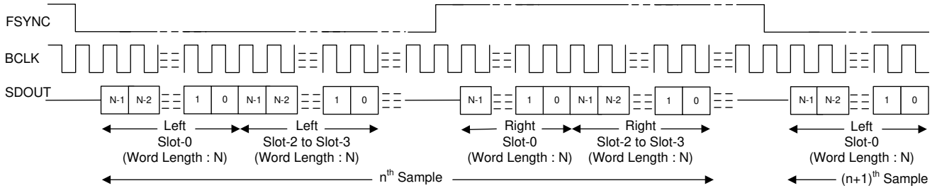
图 7-8. I 2 S Protocol Timing (TX_OFFSET = 0 and BCLK_POL = 1)
