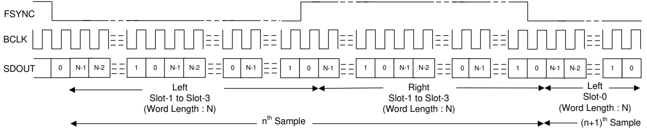
图 7-7. I 2 S Protocol Timing (No Idle BCLK Cycles, TX_OFFSET = 0)
