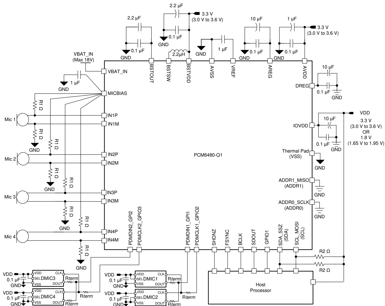
图 9-1. Four-Channel Analog Microphone and Four-Channel Digital Microphone Simultaneous Recording
