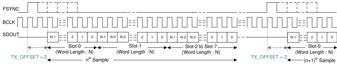
图 8-3. TDM Mode Protocol Timing (TX_OFFSET = 2)
