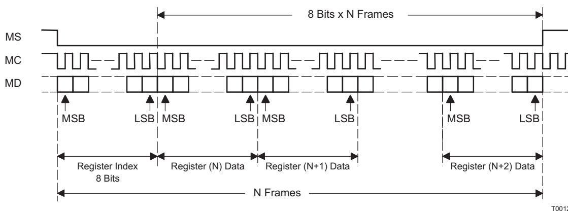
Figure 18. Register Write Operation
