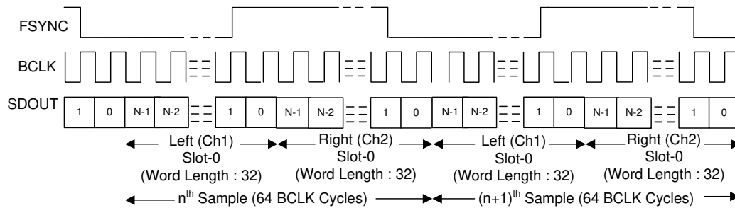
图 8-6. I²S Protocol Timing in Master Mode
