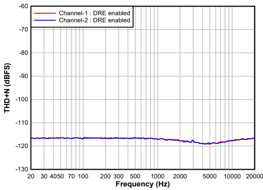
图 7-3. Differential Input: DR vs Input Frequency With DRE Enabled
