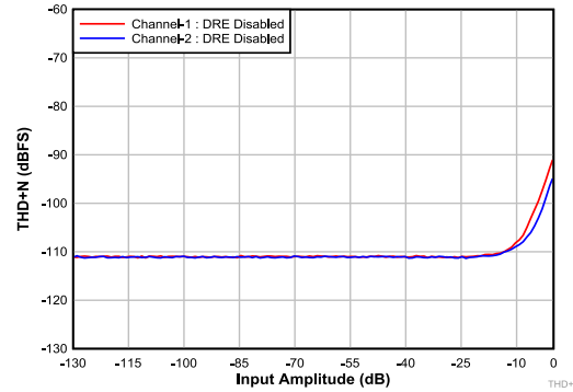
图 7-2. Differential Input: THD+N vs Input Amplitude With DRE Disabled
