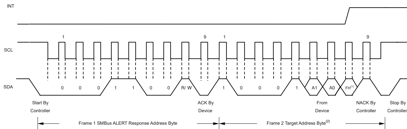
图 8-7. Timing Diagram for SMBus Alert Response
