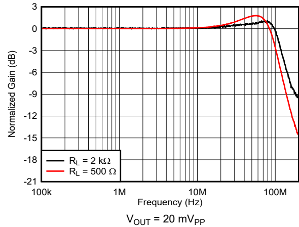
图 7-2. Small-Signal Frequency Response vs Output Load
