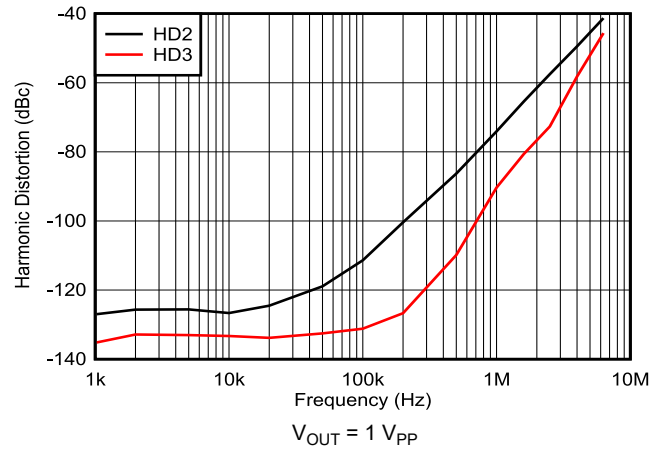
图 7-32. Harmonic Distortion vs Frequency
