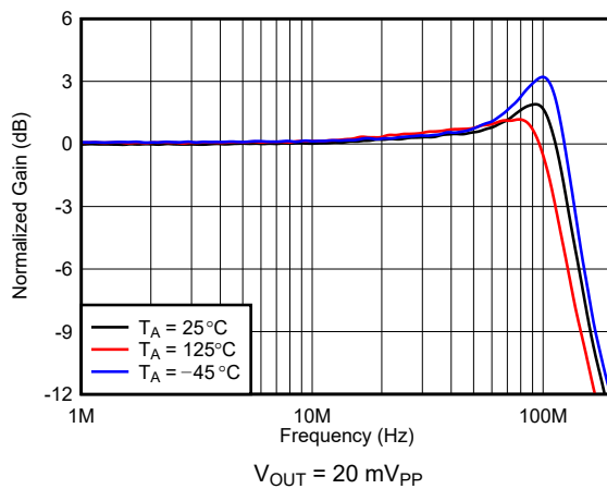
图 7-5. Frequency Response vs Ambient Temperature
