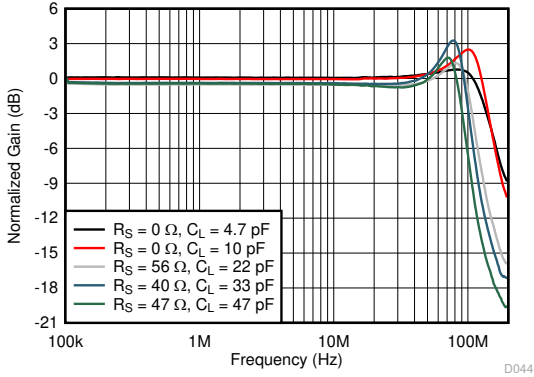
See 图 8-1 and 图 7-1, V_O = 20\text{ mV}_{PP} , gain = 1 V/V, R_F = 0\ \Omega
