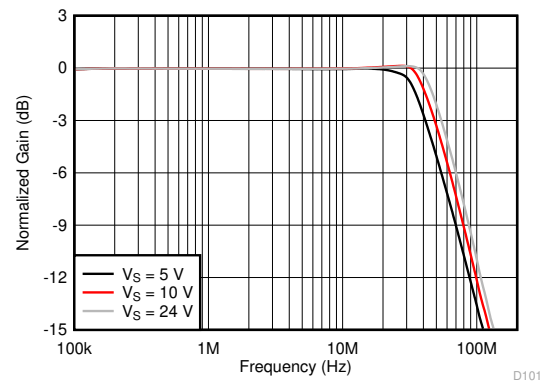
See 图 8-1, gain = 1 V/V, R_F = 0\ \Omega 图 6-43. Large-Signal Response vs Supply Voltage
