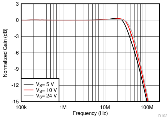
See 图 8-1, gain = 2 V/V 图 6-44. Large-Signal Response vs Supply Voltage
