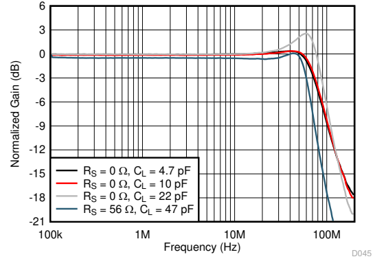
See 图 8-1 and 图 7-1, V_O = 20\text{ mV}_{PP} , gain = 2 V/V
