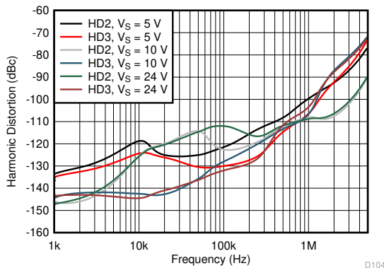
See 图 8-2, gain = -1 V/V 图 6-46. Harmonic Distortion vs Frequency vs Supply Voltage
