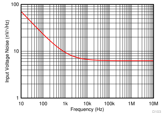
Measured then fit to ideal 1/f model 图 6-47. Input Voltage Noise Density vs Frequency
