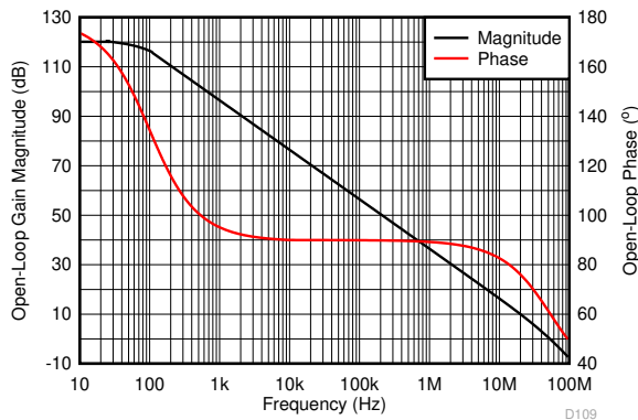
图 6-42. Open-Loop Gain and Phase vs Frequency
