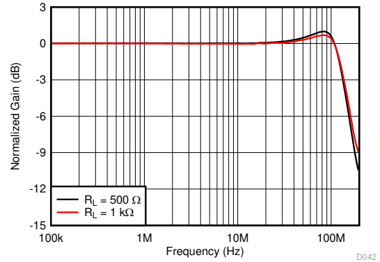
See 图 8-1, V_O = 20\text{ mV}_{PP} , gain = 1 V/V, R_F = 0\ \Omega
