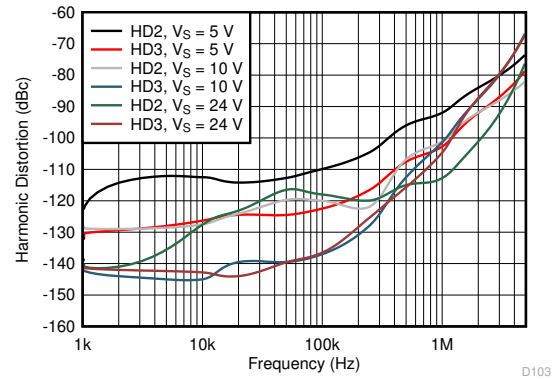
See 图 8-1, gain = 2 V/V 图 6-45. Harmonic Distortion vs Frequency vs Supply Voltage
