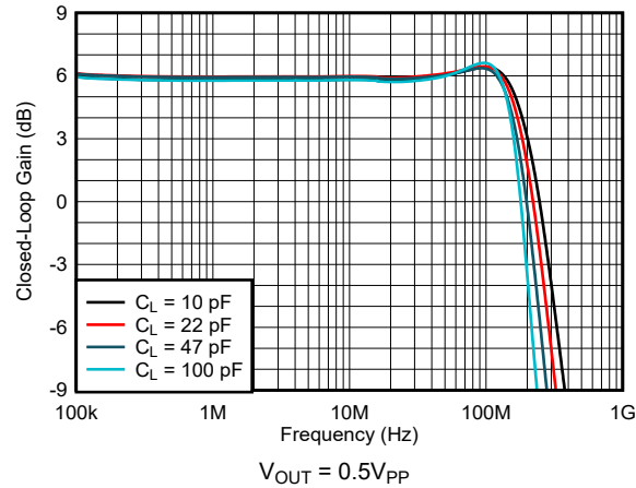
图 6-36. Frequency Response vs Capacitive Load
