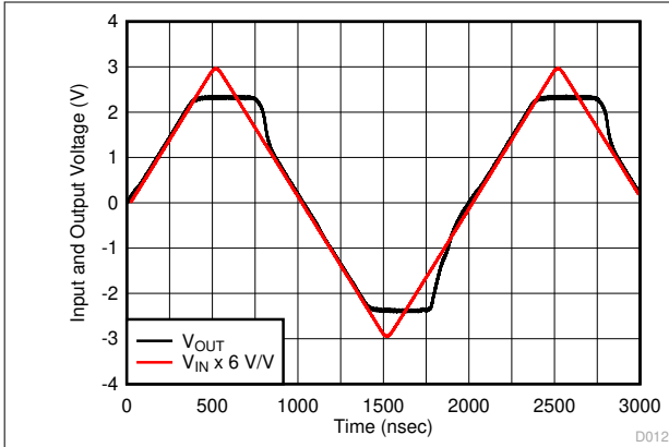
图 7-13. Output Overdrive Recovery
