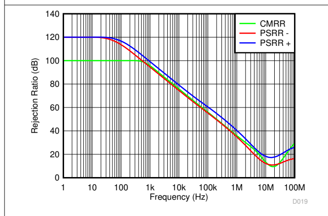
图 7-11. Rejection Ratio vs frequency
