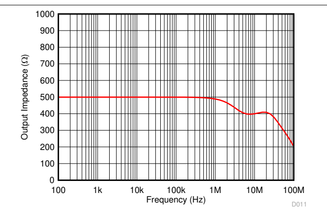
图 7-12. Open Loop Output Impedance vs Frequency
