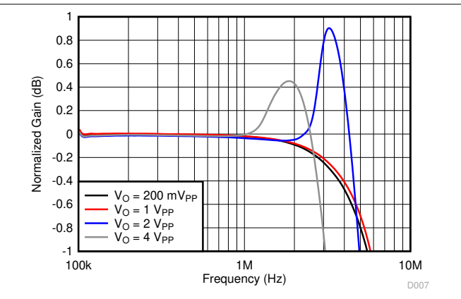
图 7-8. Large-Signal Response Flatness vs Frequency
