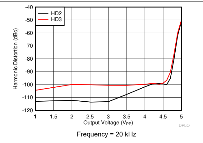
图 7-10. Harmonic Distortion vs Output Voltage
