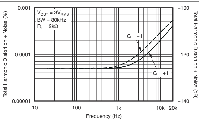
图 6-11. THD+N Ratio vs Frequency
