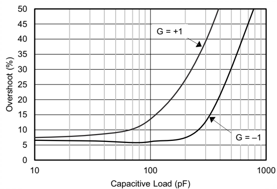
图 5-17. Small-Signal Overshoot vs Load Capacitance
