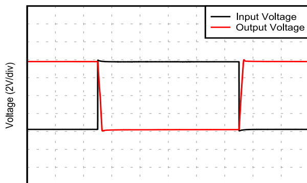
Time (20µs/div) G = -1, 4V 阶跃
