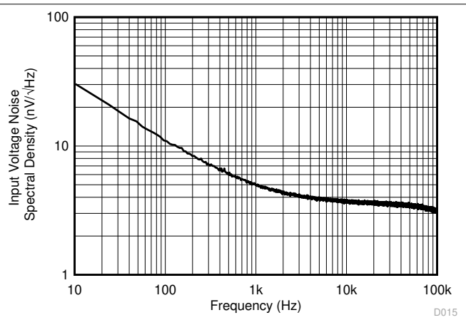
图 7-16. Input Voltage Noise Spectral Density vs Frequency
