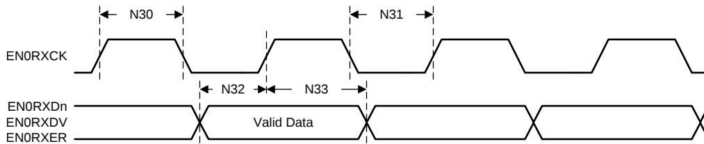
图 5-38. 100-Mbps MII Receive Timing
