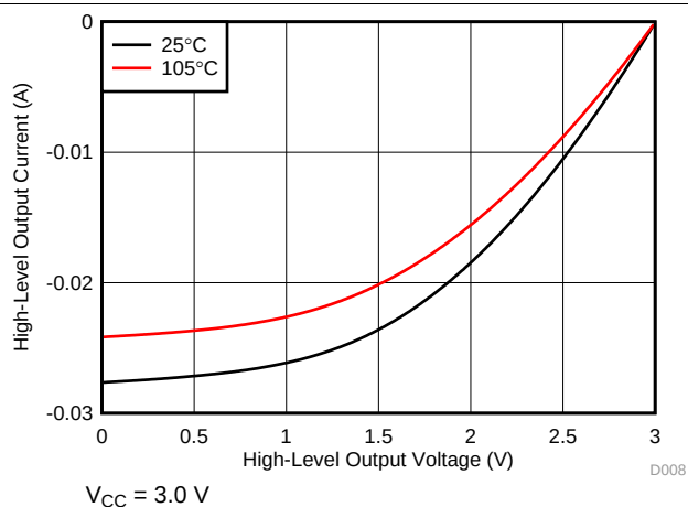
Figure 4-8. Typical High-Level Output Current vs High-Level Output Voltage
