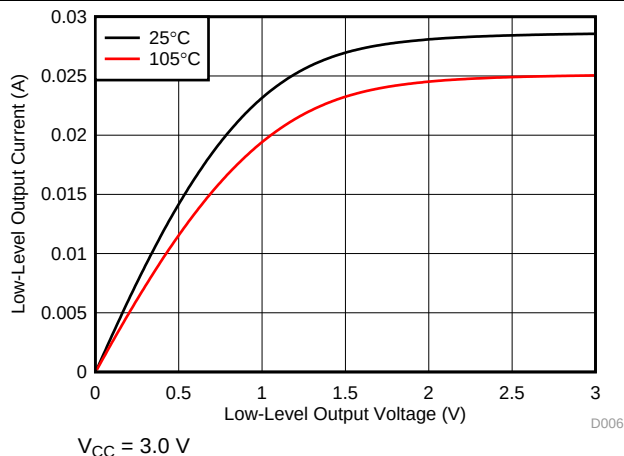
Figure 4-6. Typical Low-Level Output Current vs Low-Level Output Voltage
