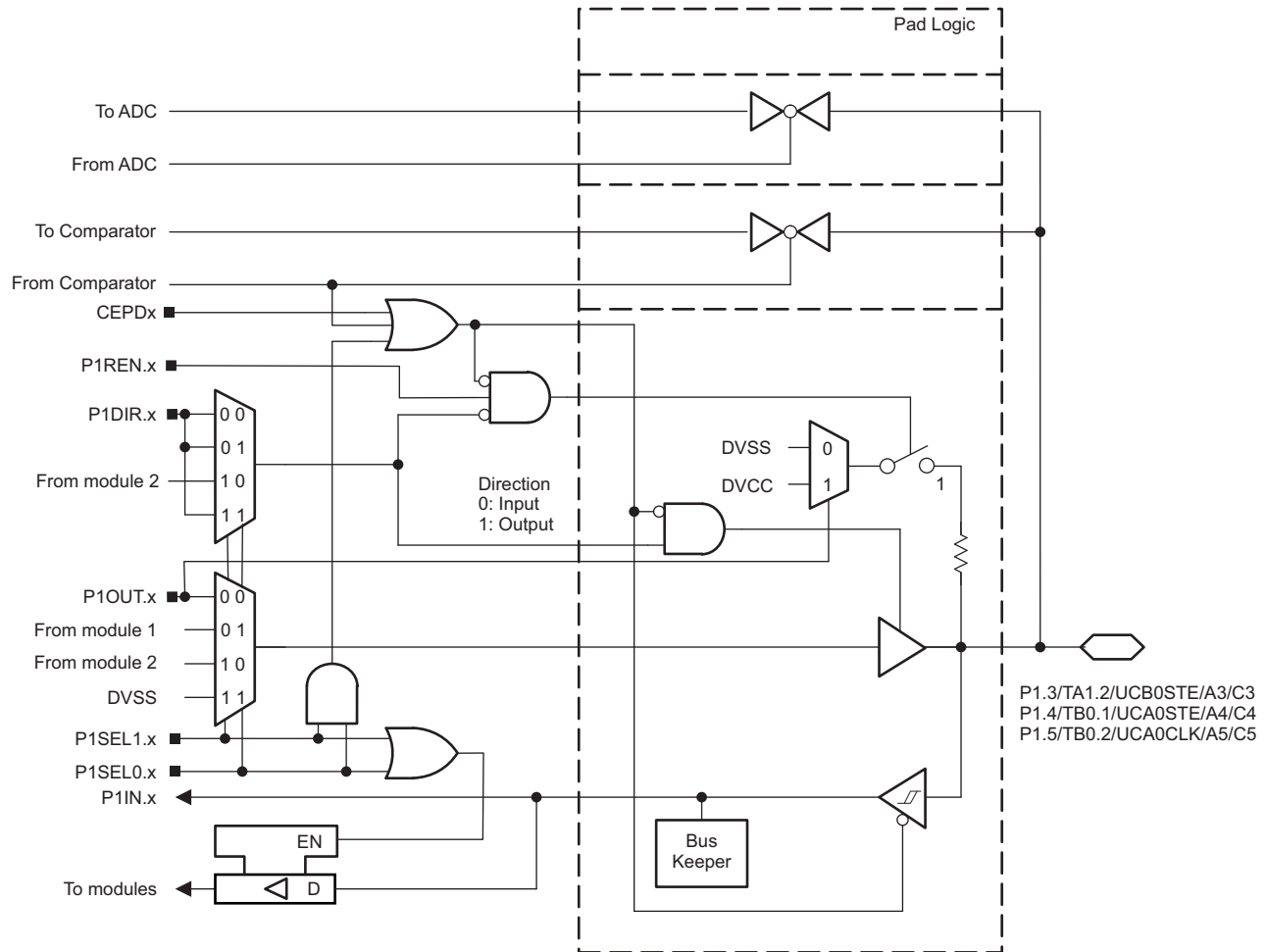
图 5-3. Port P1 (P1.3 to P1.5) Diagram
